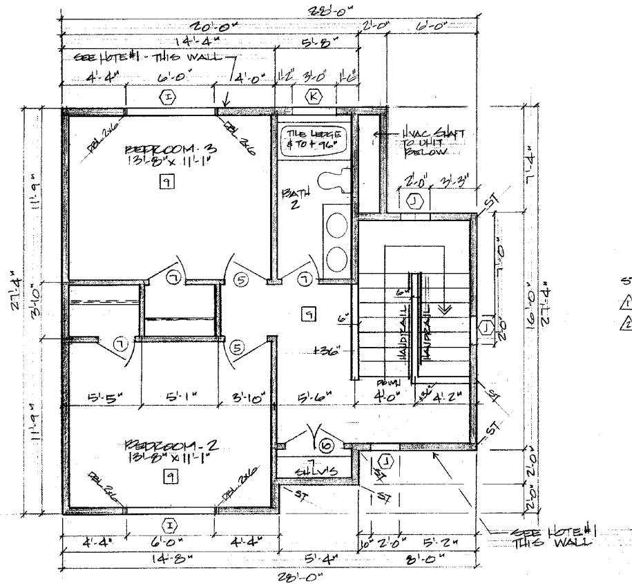
UPPER FLOOR - FLOOR PLAN
